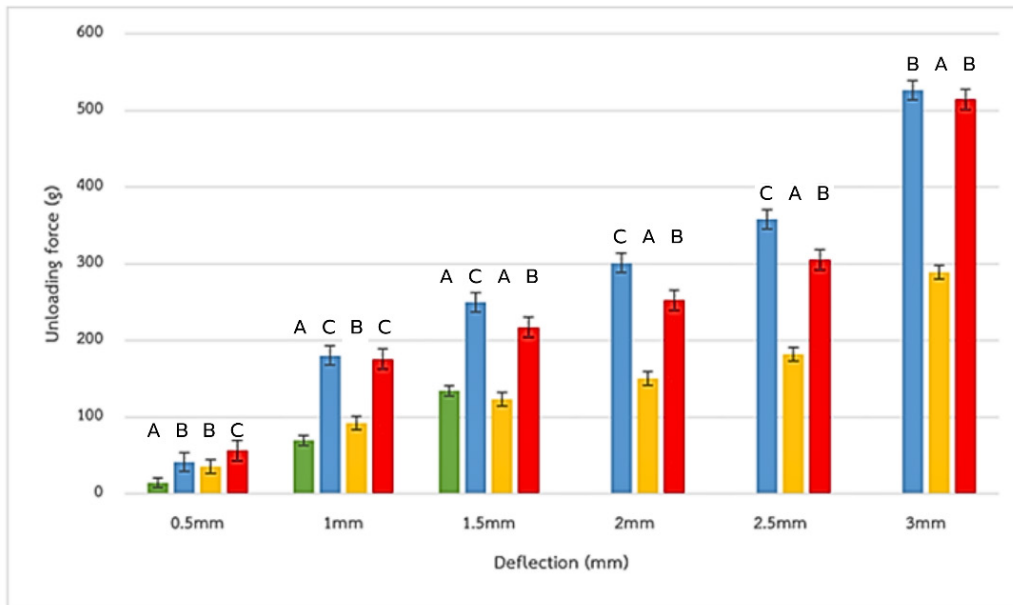
Figure 2 Mean unloading force of 4 types of wire at various levels of deflection. In each deflection point, the same alphabet means no statistically significant difference ( p > 0.05 ). While different alphabets represent statistically significant differences ( p < 0.05 ) comparing only in the same deflection point.
